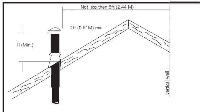
MINIMUM HEIGHT FROM ROOF TO LOWEST DISCHARGE OPENING
