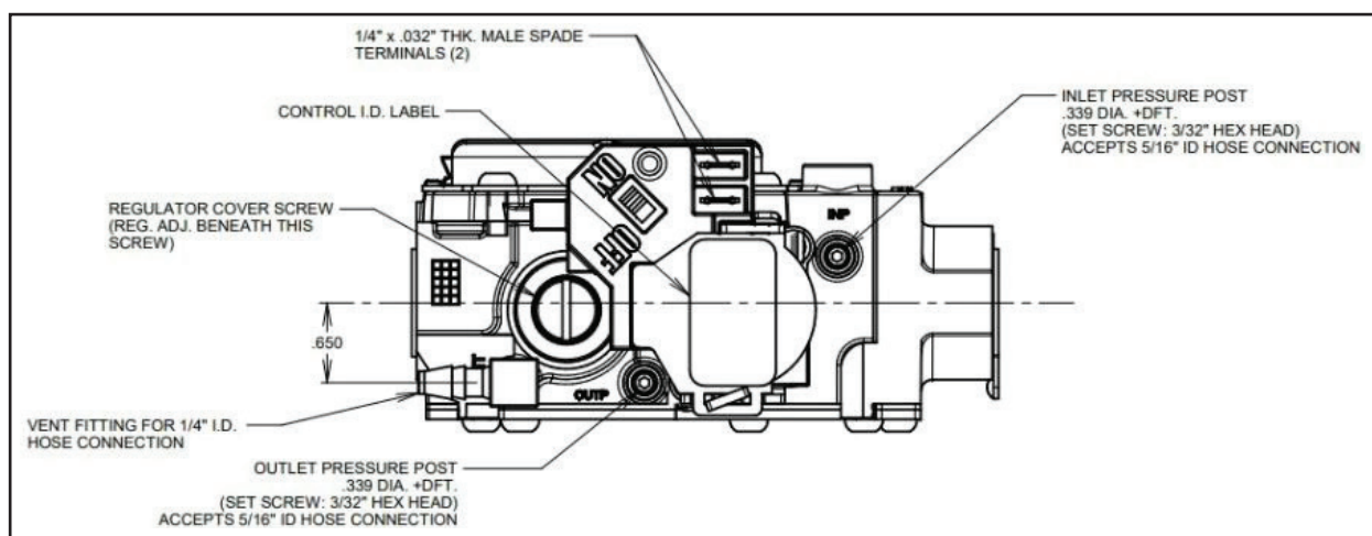
Figure 12 - Gas Valve Details Models HSU100 through 200
